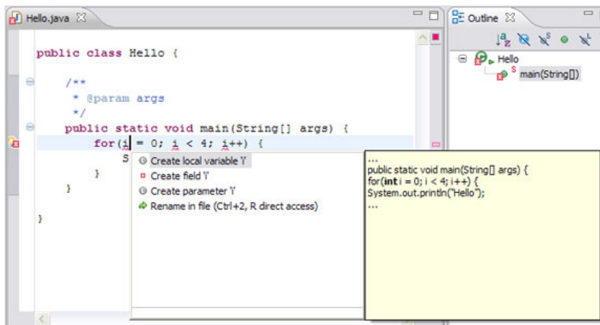
Figure 5. Quick Fix suggestions
